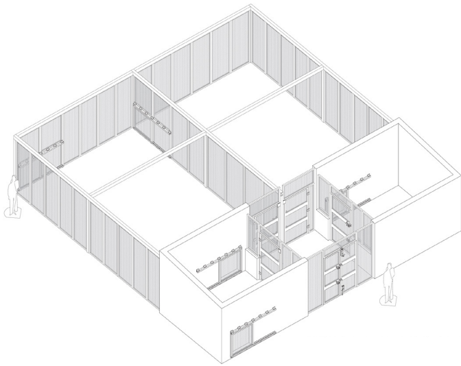
Saola habitat holding shelter
